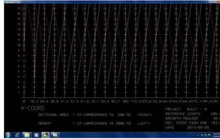
Figure 7: The Sectional Area Curves Obtained from Tribon
